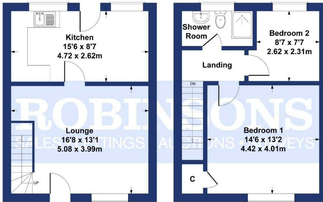
GROUND FLOOR
